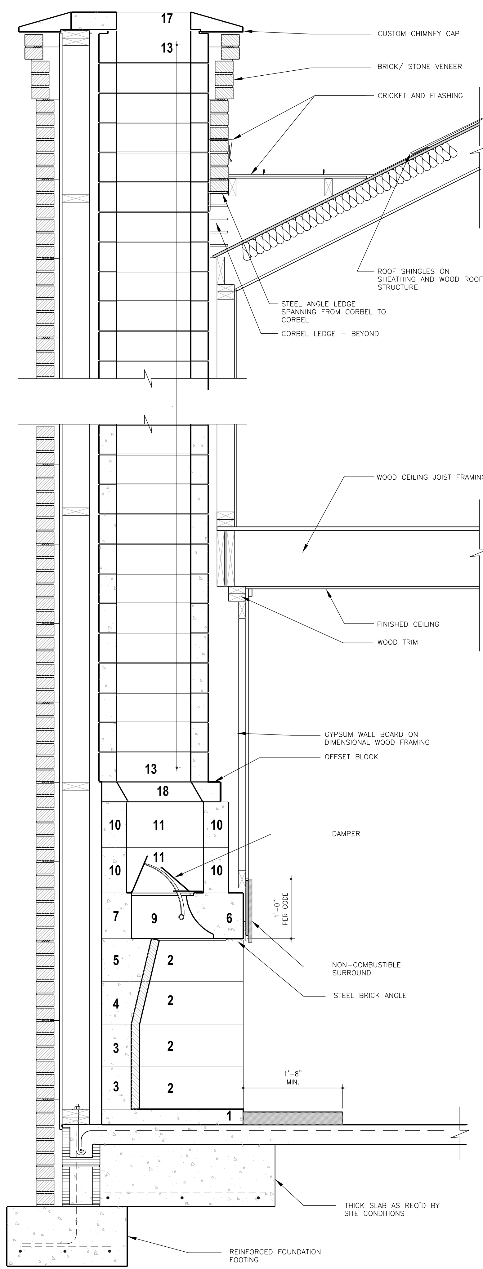
SECTION- BRICK/ STONE CHIMNEY W/ OFFSET BLOCK
