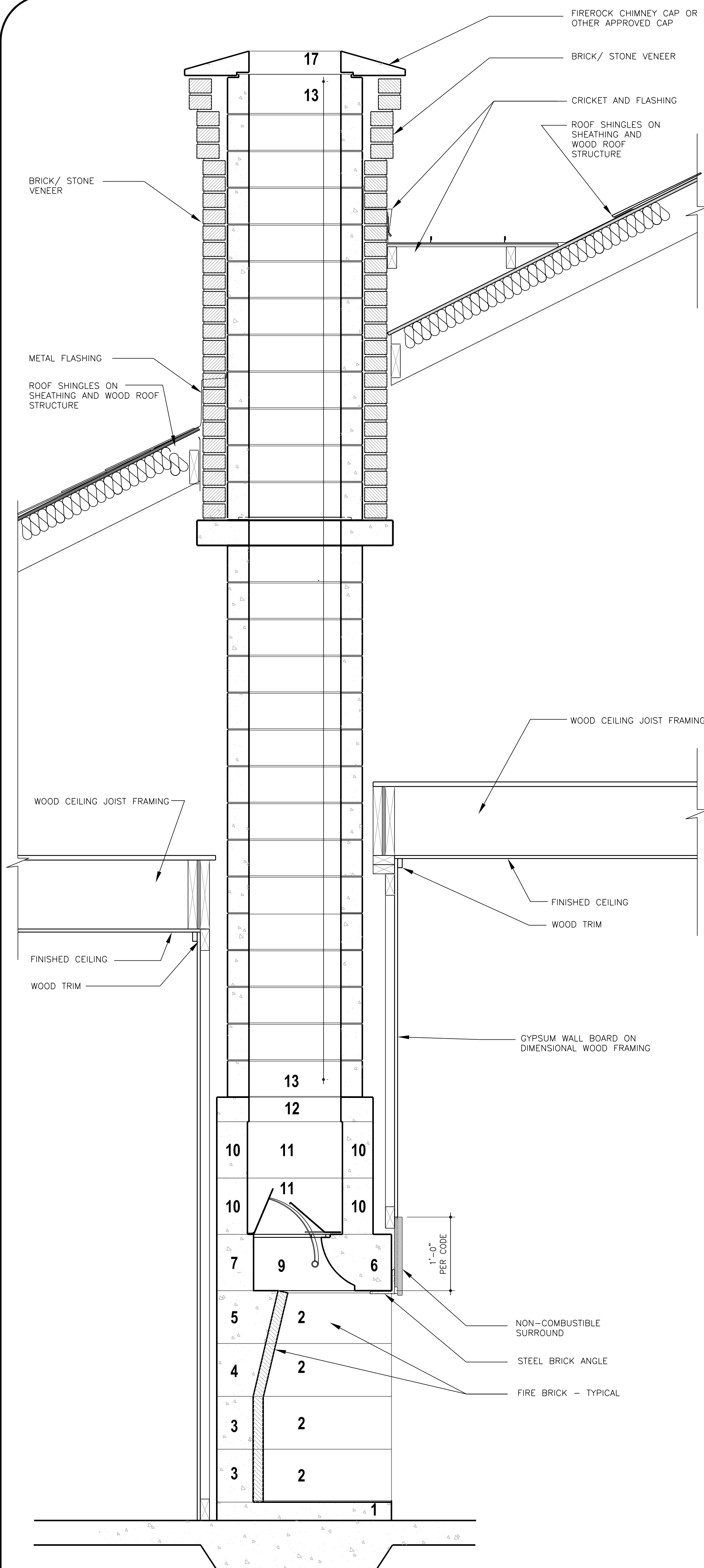
SECTION- BRICK/ STONE ON ENTIRE FIREPLACE
